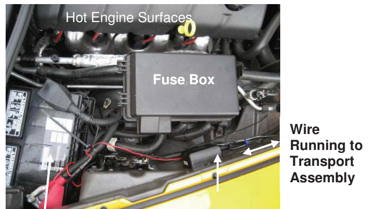
Radio receiver mounted behind Fuse Box (or behind the battery in other installations)
